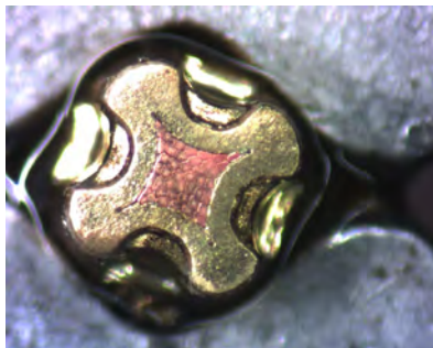
4/8-indent crimp
